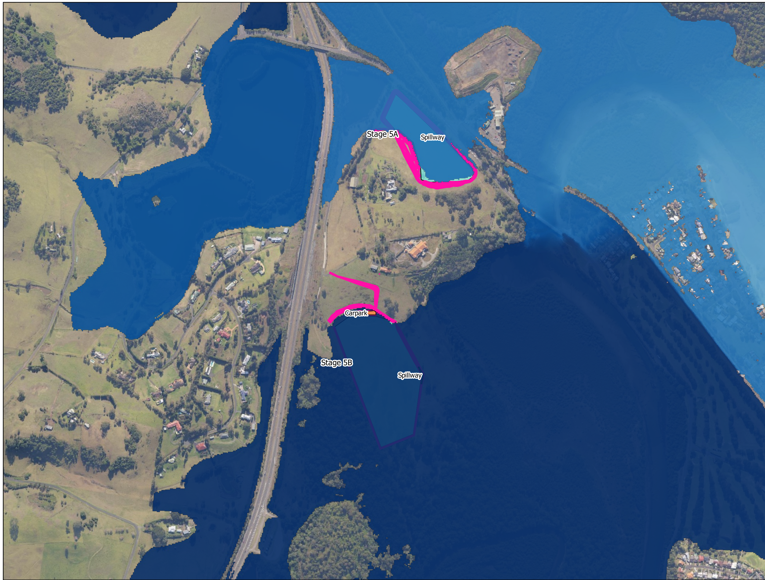
FIG 28. PMF Flood height, proposed conditions.
