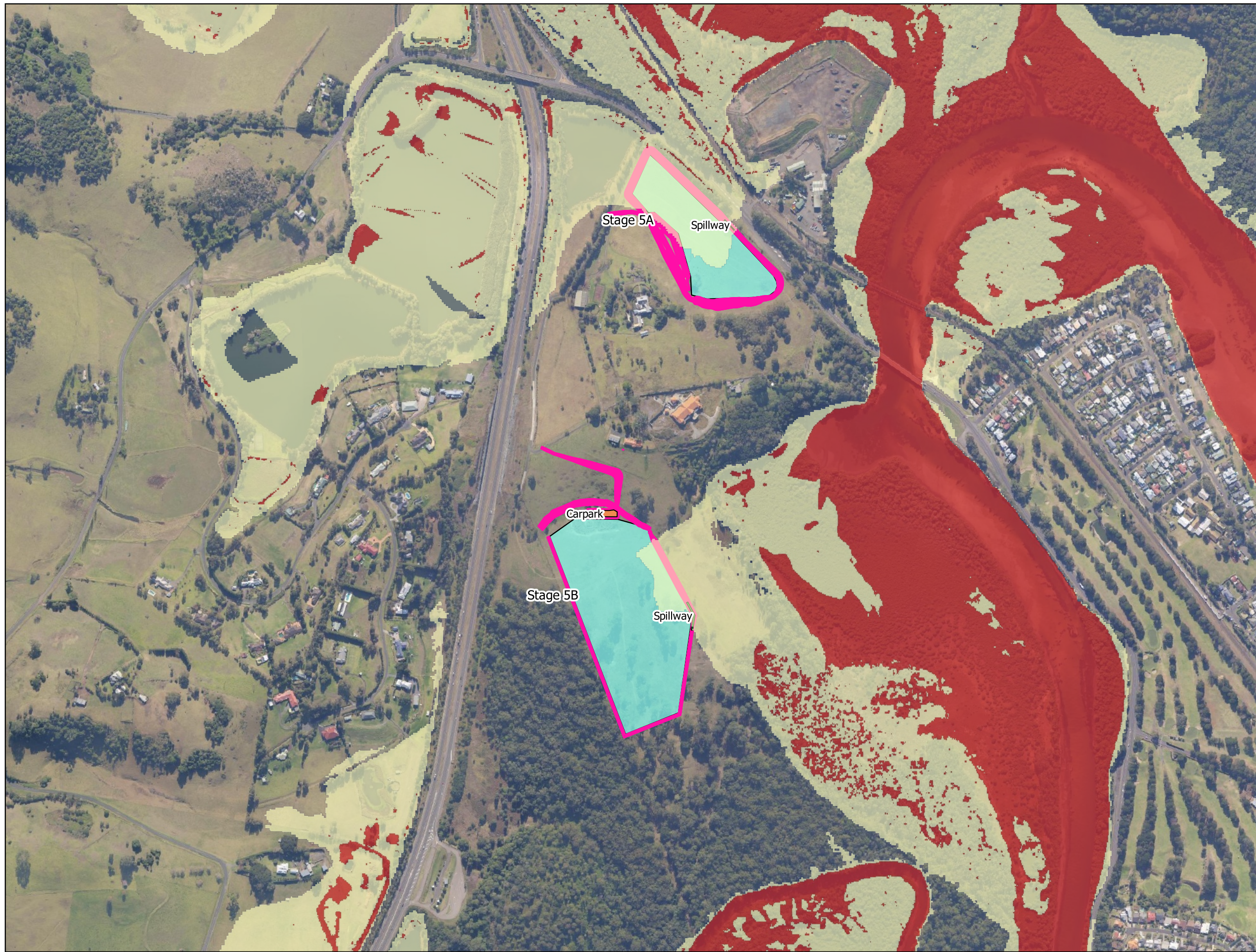
FIG 15. 20y ARI flood hazard, existing conditions.
