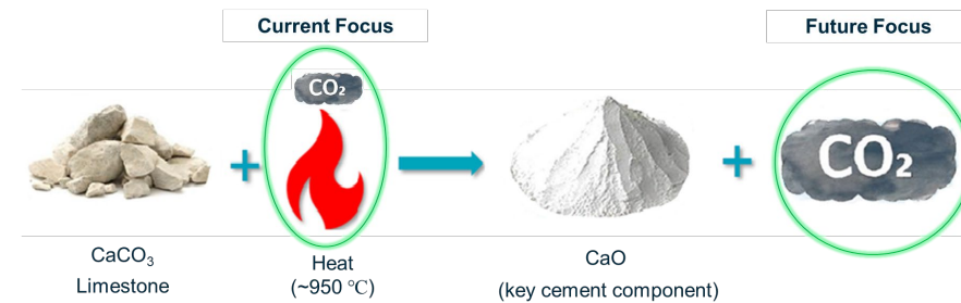
Calcination process
